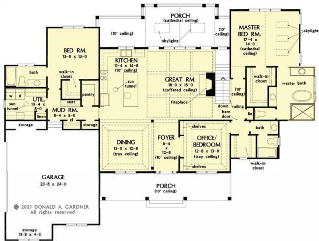
FLOOR PLAN PLAN NO. 1610
