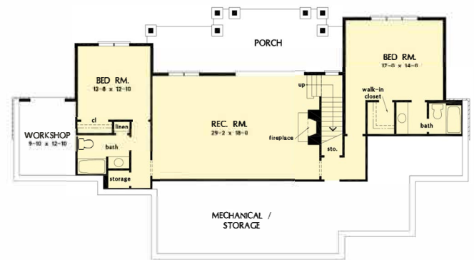
FLOOR PLAN PLAN NO. 1610 D
