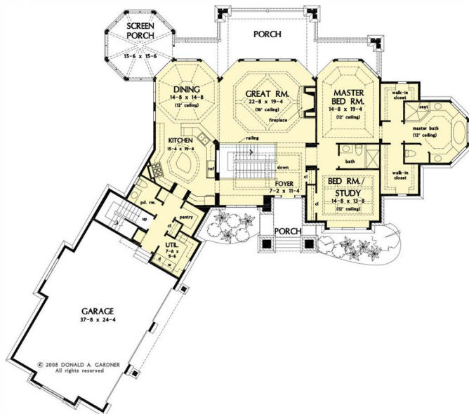
FLOOR PLAN PLAN NO. 5020
