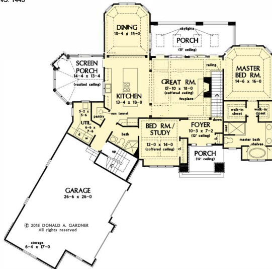
FLOOR PLAN PLAN NO. 1445
