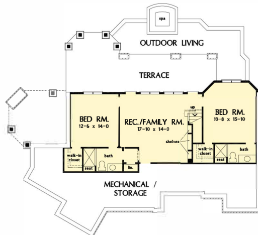
FLOOR PLAN PLAN NO. 1445
