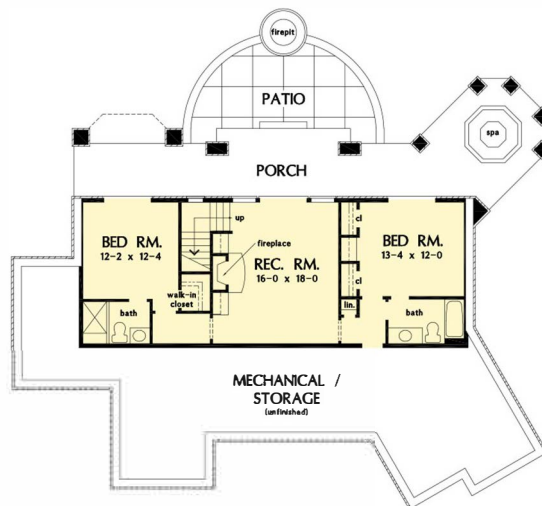
FLOOR PLAN PLAN NO. 1301 D
