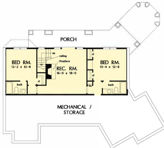
FLOOR PLAN PLAN NO. 1320
